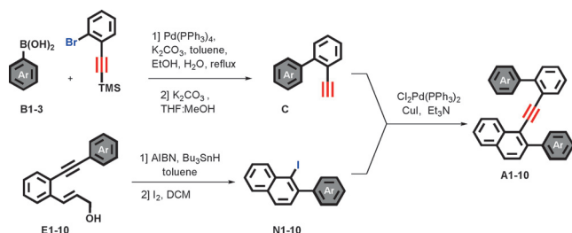
Scheme 2. The synthetic route for preparing the alkynyl precursors of helicenes A1–A10 .
